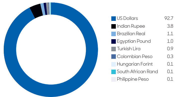
Currency breakdown (%)
